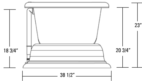
Rough-In Plumbing Measurements
